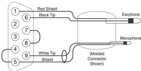
Figure 2-1: Motorola Radios
