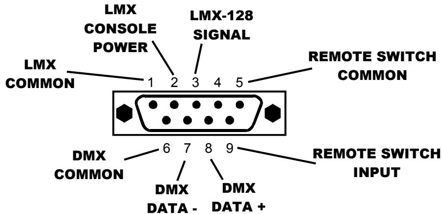
I/O CONNECTOR 9 PIN MALE (DB9) Used on rear of chassis
