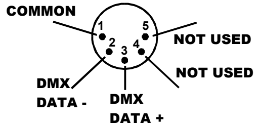
DMX-512 CONNECTOR 5 PIN MALE XLR Used on adapter cable
