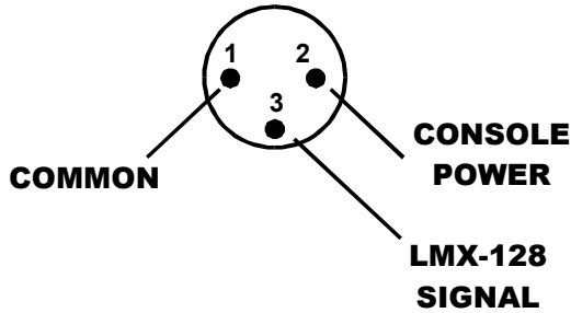
MULTIPLEX (LMX) CONNECTOR 3 PIN MALE XLR Used on rear of chassis
