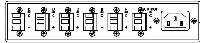
model 521E-TB REAR TWO PART SEPARATING TERMINAL BLOCK NOTE: MAXIMUM NUMBER OF INPUTS IS REDUCED FROM 6 TO 5
